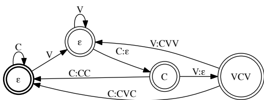
Figure 4: An SFST for the copy process of Rotuman CV-metathesis.
